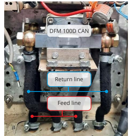
Differential fuel flow meter installation
