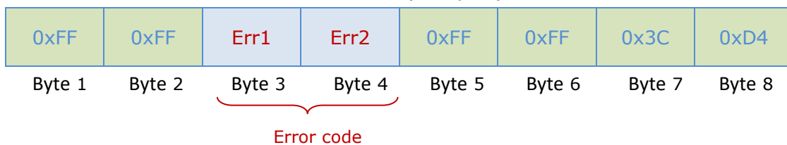
Figure 15 — Composition of a GNOM DP CAN error message
