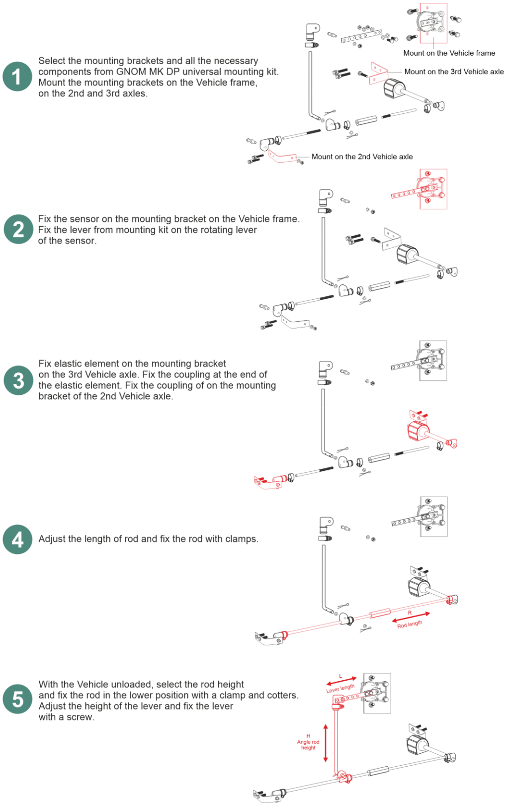
Figure 24 — Stages of mounting GNOM DP according to the typical scheme for a three-axial Vehicle
