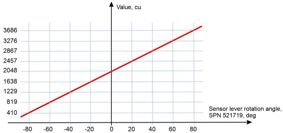
Figure 14 — Graph of GNOM DP CAN output data dependence on the sensor lever rotation angle
