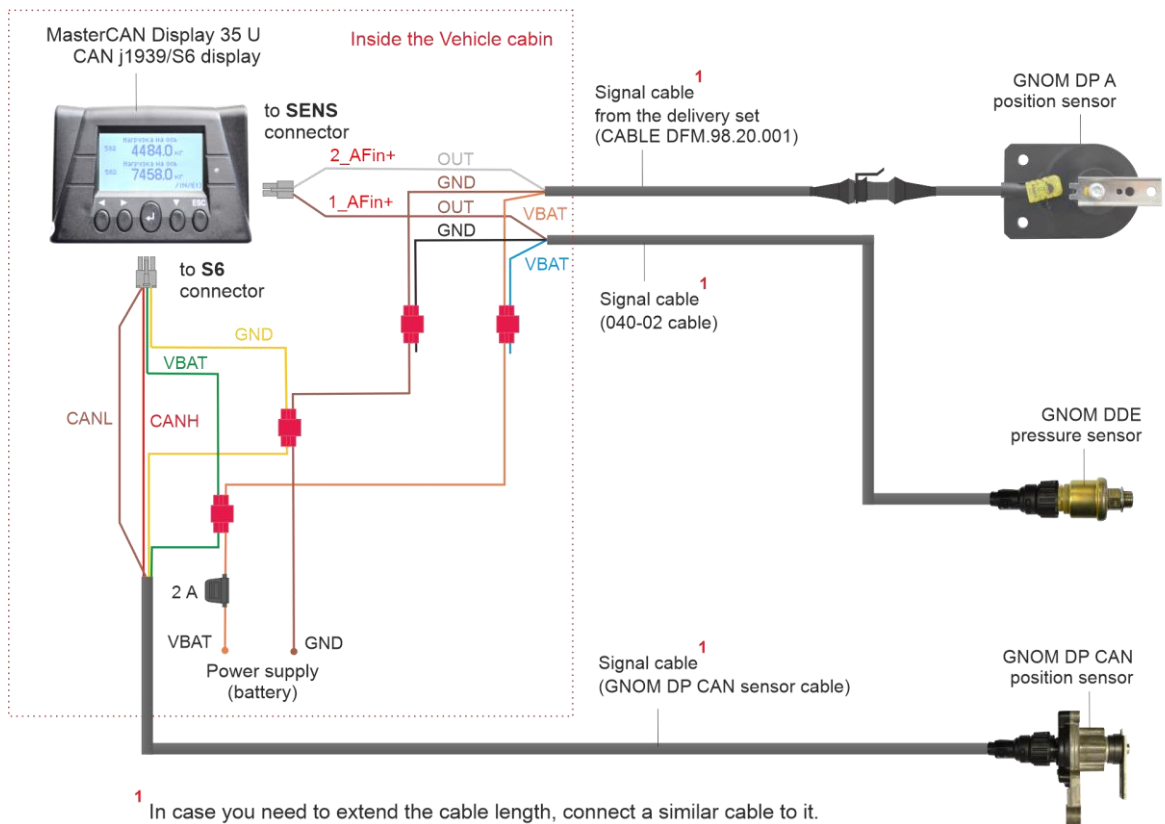
Figure 44 — Example of the connection diagram of two GNOM DP A and GNOM DDE analog sensors and one GNOM DP CAN digital sensor to MasterCAN Display 35 U
