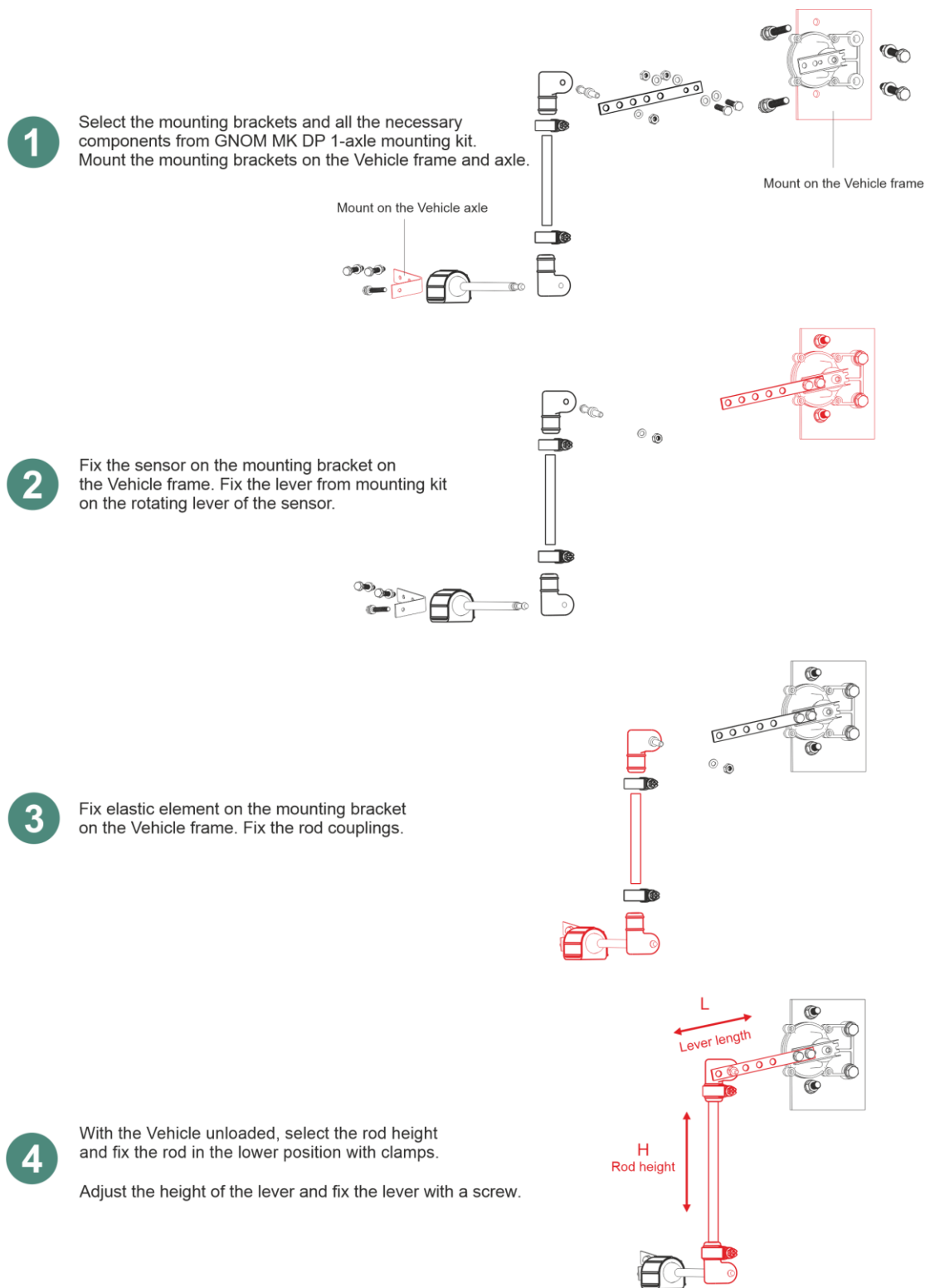
Figure 22 — Stages of mounting GNOM DP according to the typical scheme for a two-axial Vehicle
