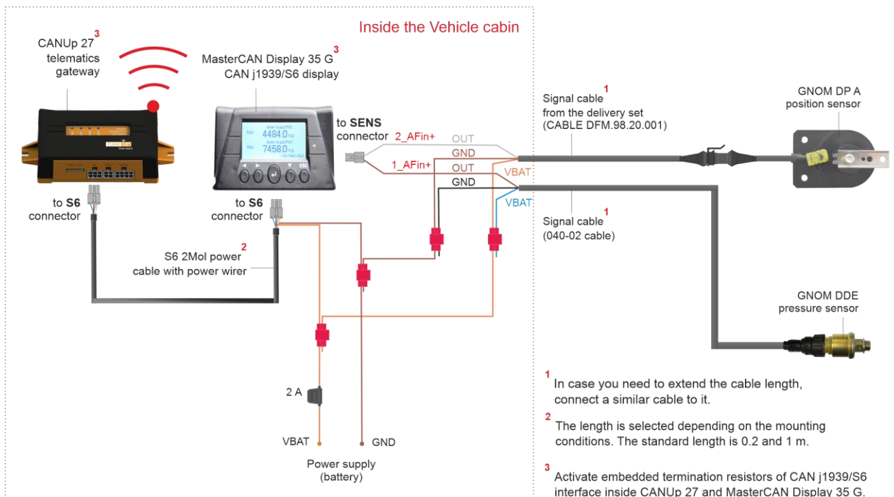
Figure D.1 — Typical scheme of the equipment connection for monitoring the axle load for a road train with a non-interchangeable semitrailer (see figure 5 )
