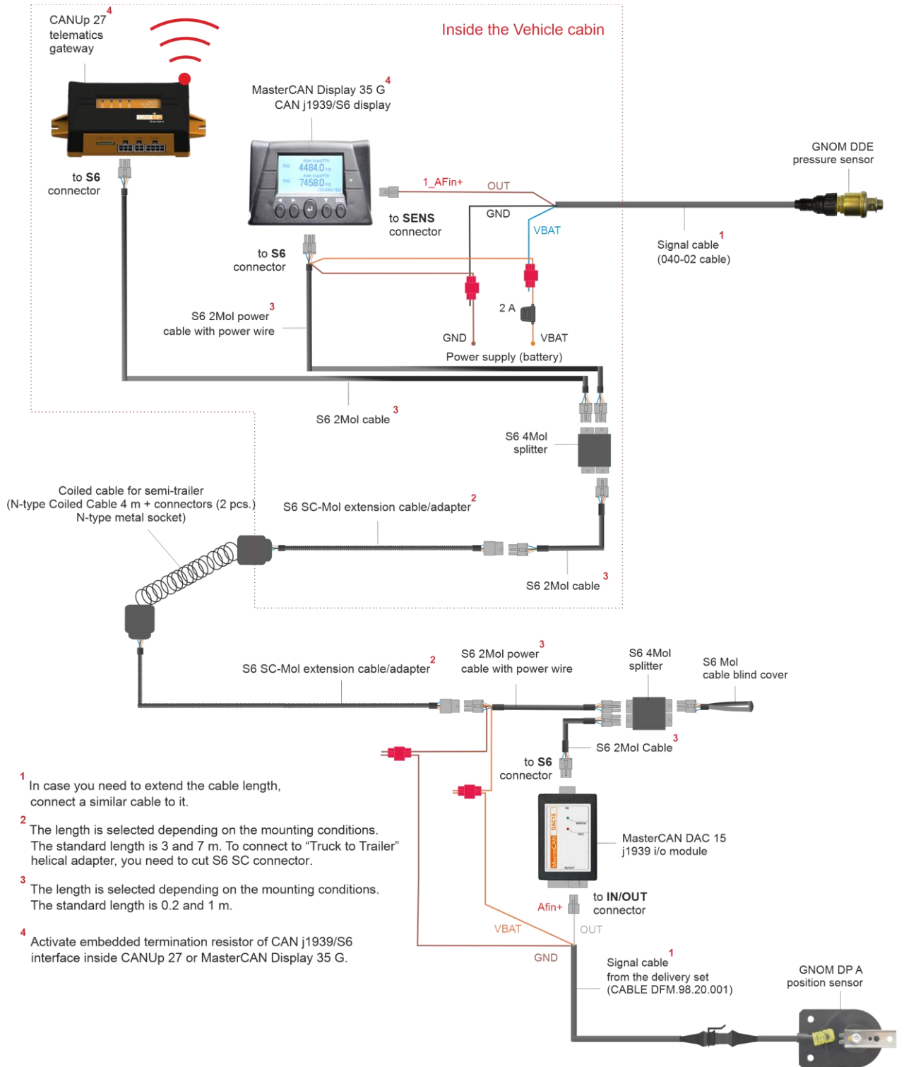
Figure D.2 — Typical scheme of the equipment connection for monitoring the axle load for a road train with a replaceable semitrailer (see figure 6 )
