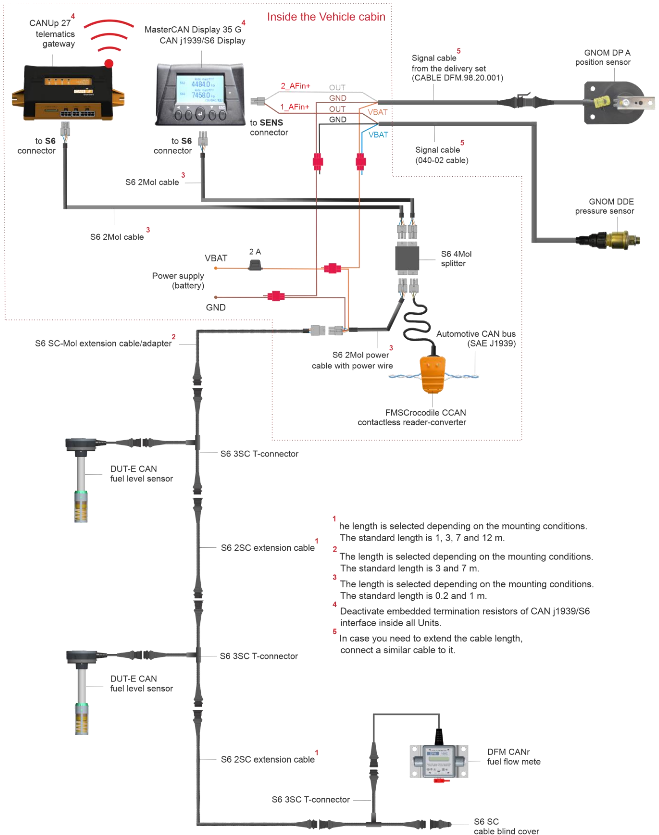
Figure 45 — Connection diagram of two GNOM sensors to MasterCAN Display 35 G together with Units and a standard Vehicle CAN bus
