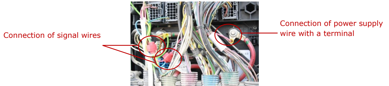
d) example of using terminals and connectors when connecting GNOM sensors
