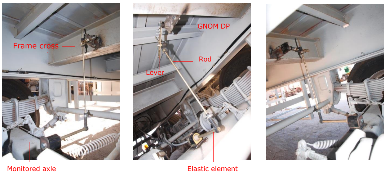
Figure 19 — Example of GNOM DP mounting location to monitor the semitrailer axle load
