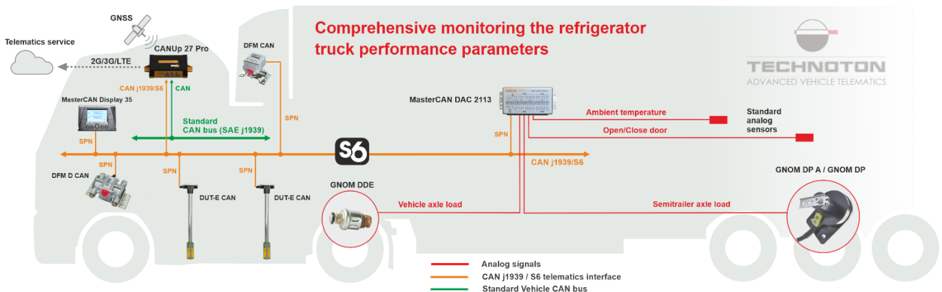
Figure 7 — Example of GNOM sensors application for monitoring axle load at comprehensive monitoring the refrigerator truck performance parameters via S6 Technology
