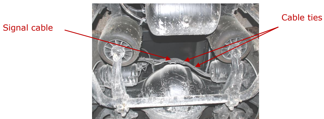
Figure 32 — Laying GNOM signal cable
