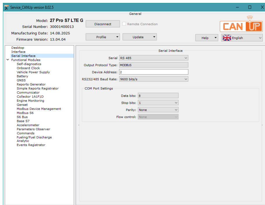
Figure 19 — Window of the CANUp 27 connection parameters configuration via serial interface
