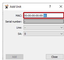
Figure 23 — Configuration of S7 Database FM for work with wireless Units using S7 Technology
