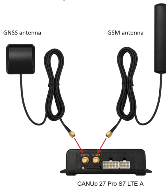
Figure 26 — Connecting External Antennas to CANUp 27 Pro S7 LTE A
