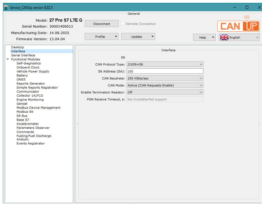
Figure 18 — Window for configuration of CANUp 27 connection parameters via CAN j1939/S6 interface
