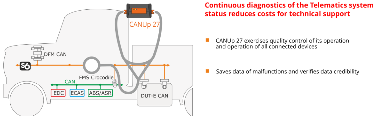
Figure 4 — Examples of CANUp 27 use on a Vehicle as part of the Telematics system
